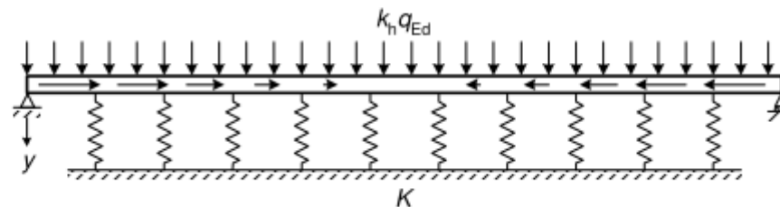
e) Free flange of purlin modelled as beam on elastic foundation. Model representing effect of torsion and lateral bending (including cross section distortion) on single span with uplift loading.
