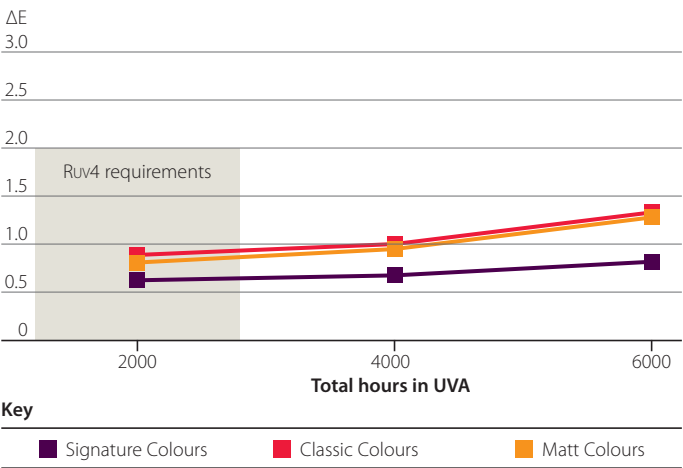
Figure 26. ΔE for Colorcoat HPS200 Ultra® in UVA
